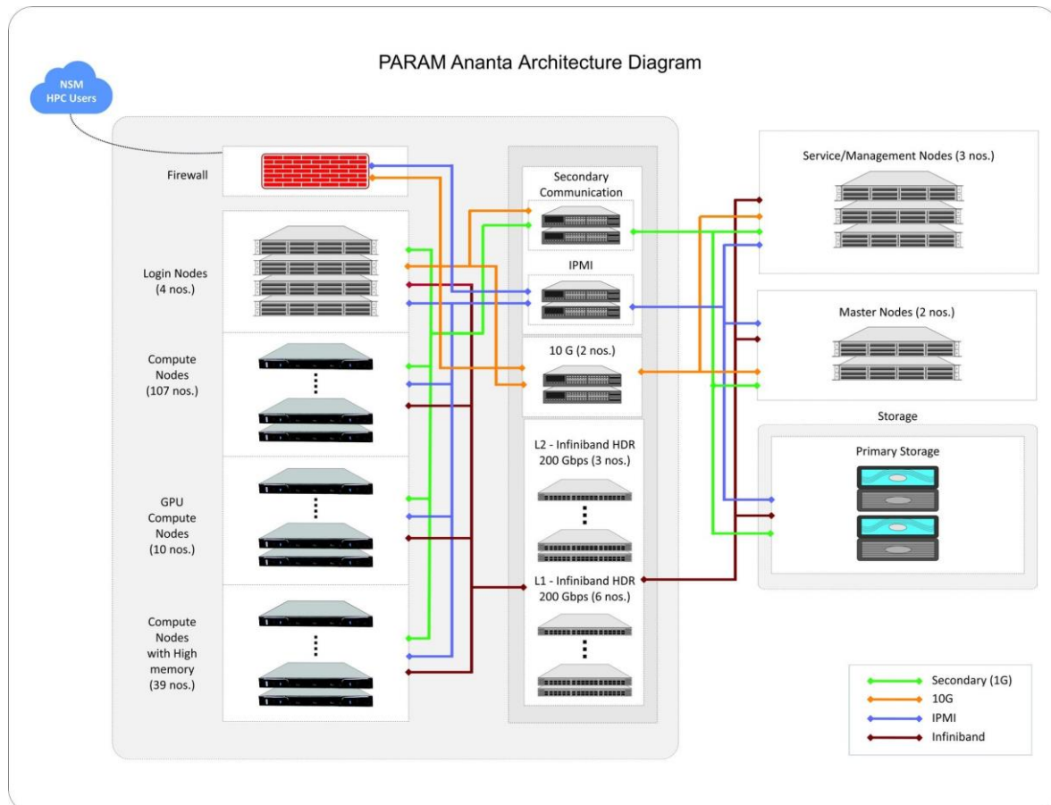
Figure 1 - PARAM Ananta Architecture Diagram
